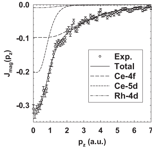
Figure 1. The experimental MCP of CeRh 3 B 2 and the best fit with atomic profiles to the experimental MCP.
