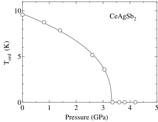
Figure 4. Pressure dependence of the magnetic ordering temperature in \text{CeAgSb}_2 . The full curve connecting the data points is a guideline.
