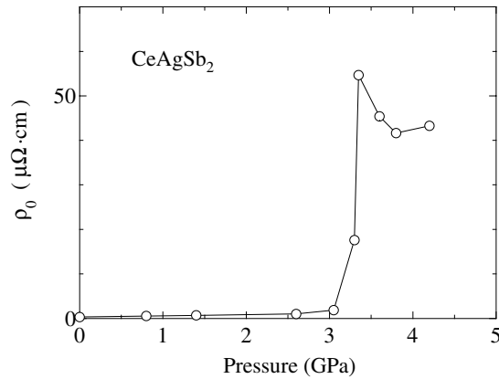
Figure 5. Pressure dependence of the residual resistivity in \text{CeAgSb}_2 .
